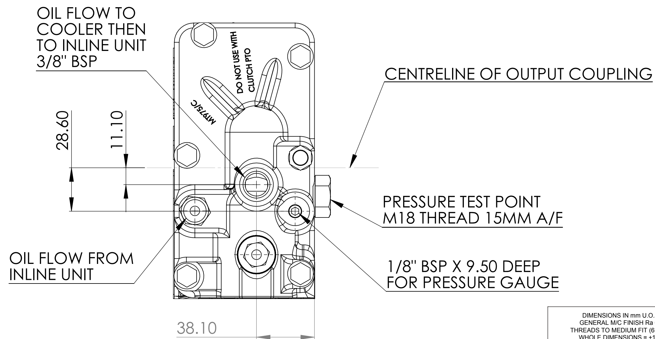
SCRAP VIEW OF VALVE BLOCK
